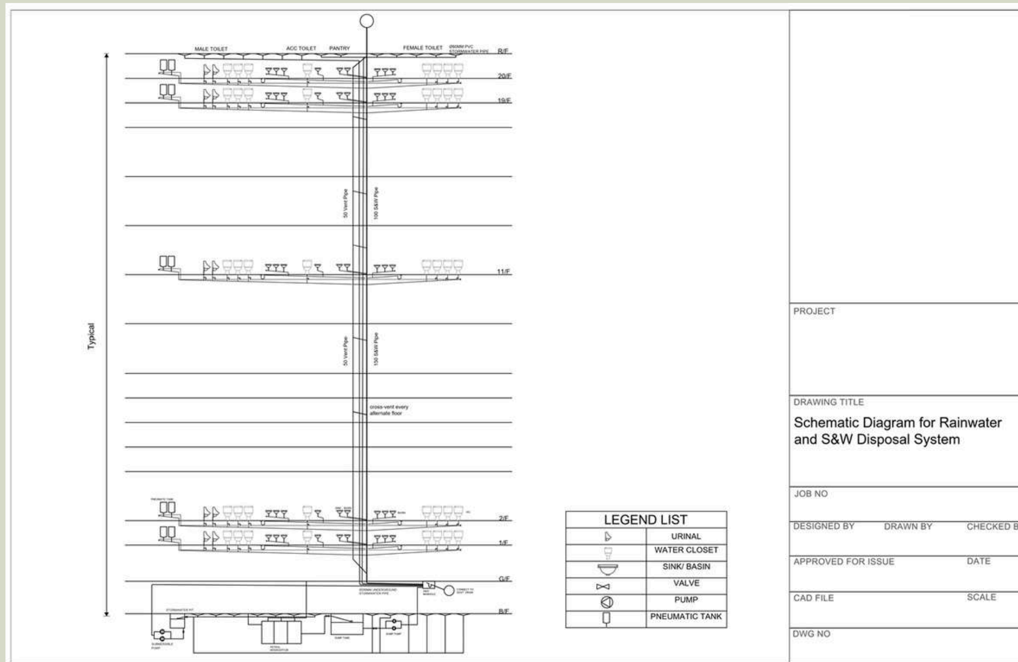
S&W and rain water system layout
