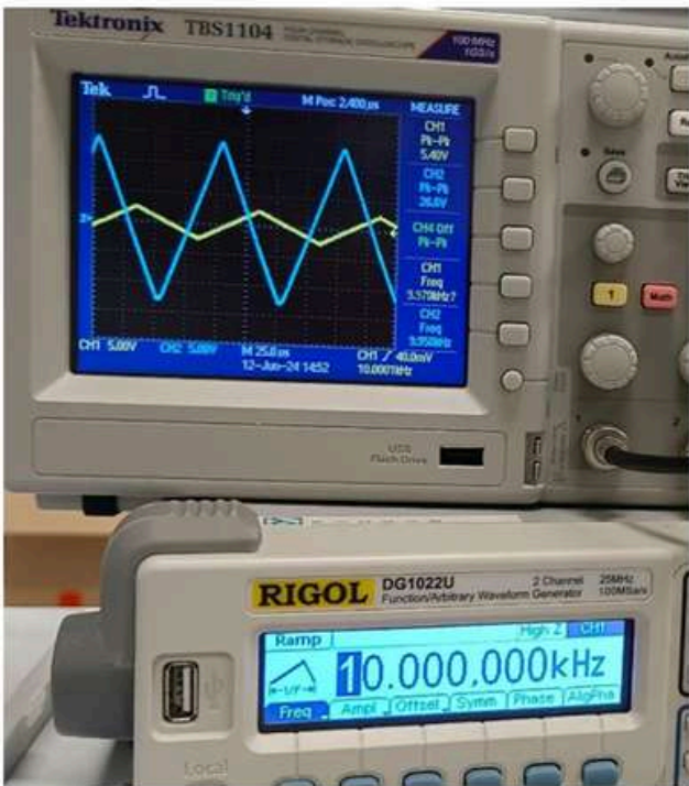
Figure 171 Waveform when frequency is 10kHz
