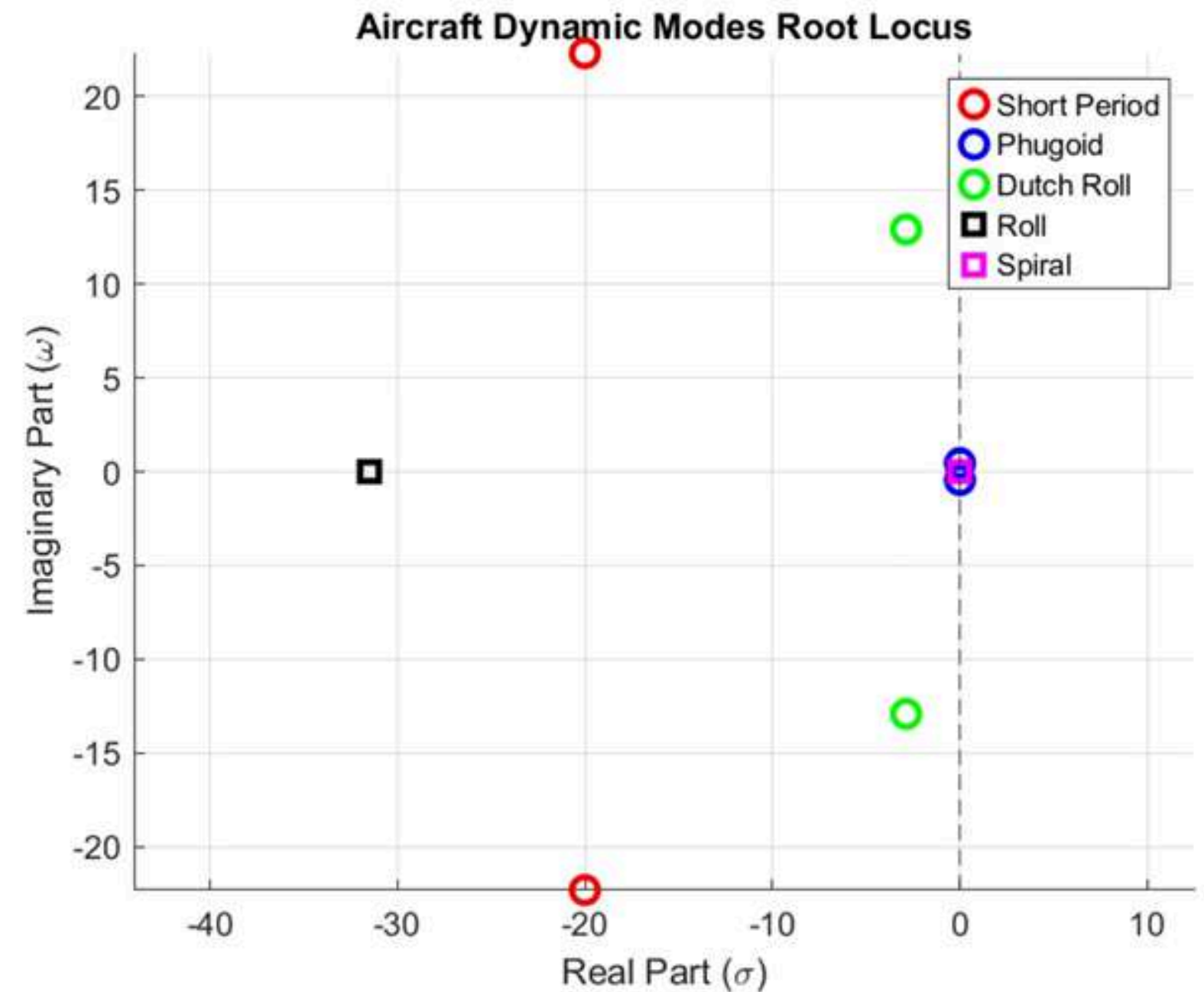
Figure 31 Aircraft Dynamic Modes Root Locus
