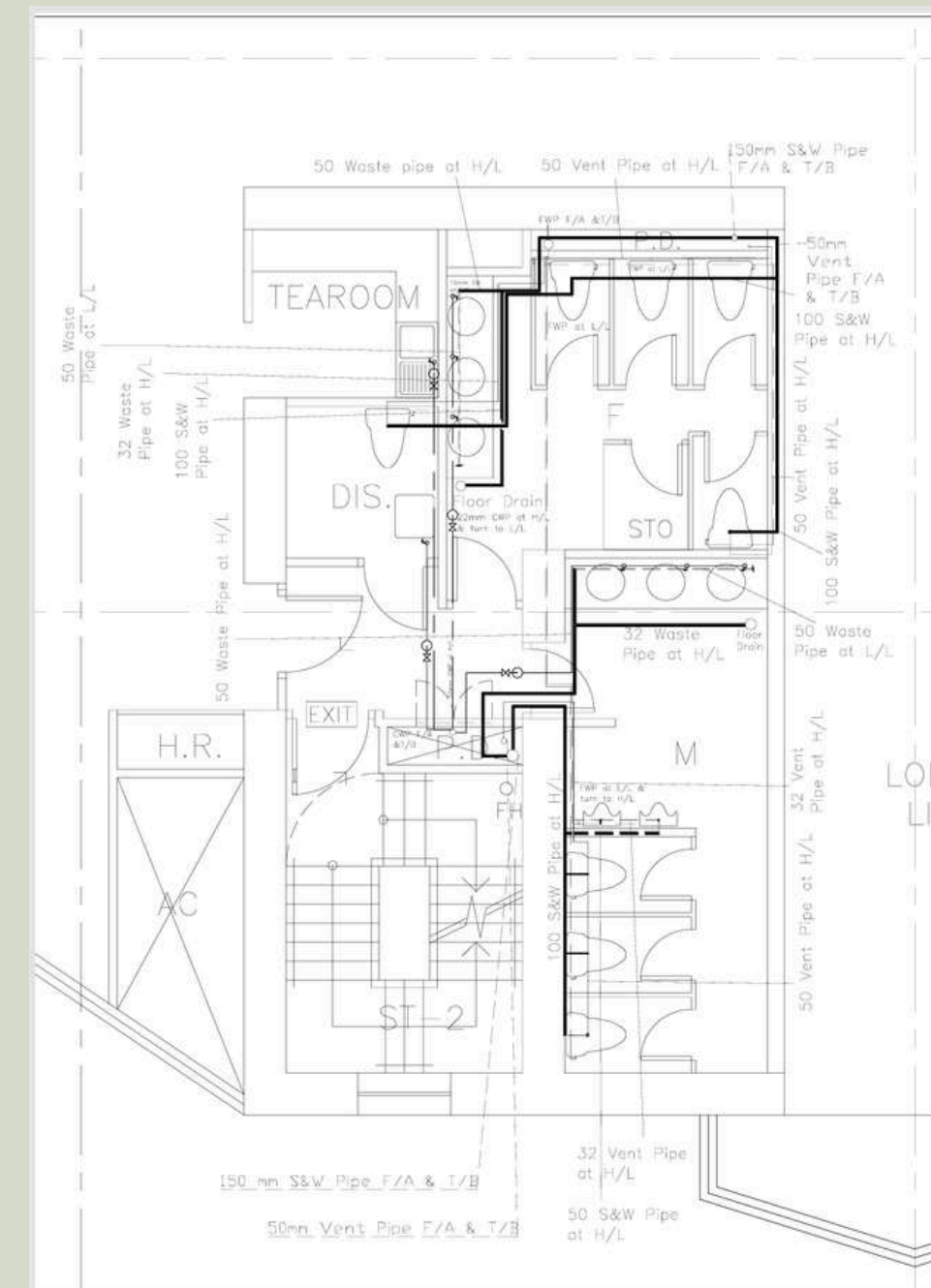
Toilet pipeline layout
