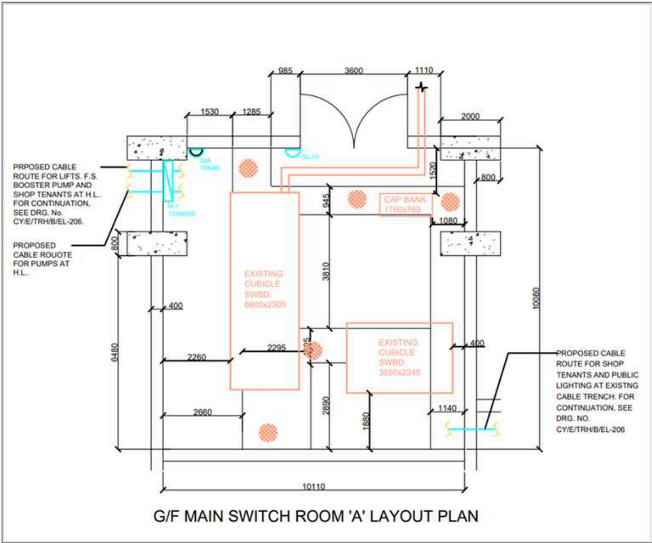
Figure 288 Task 2 of the AutoCAD assignment
